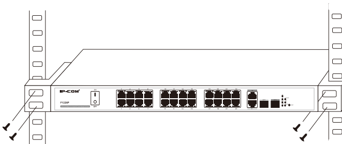
Figure 5: Install Switch in a 19-inch Rack
