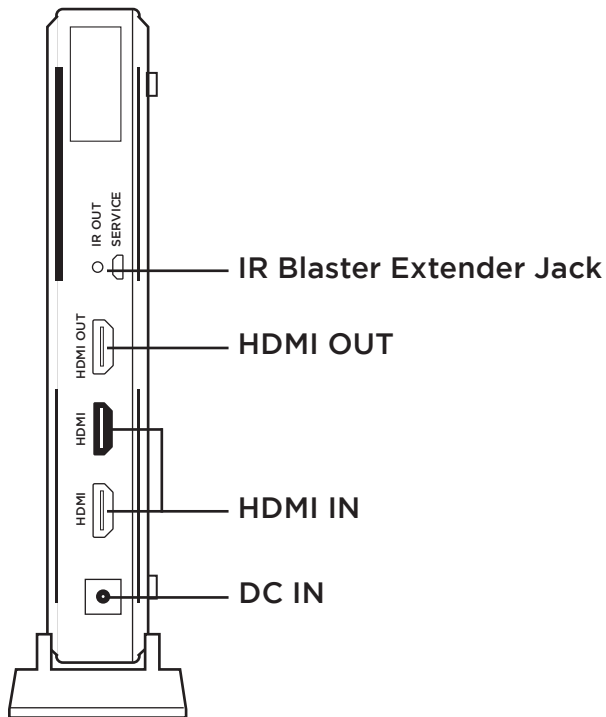
Main Unit Back Panel
