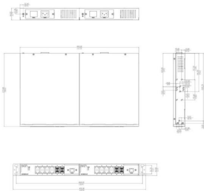
(Dual Mount)
