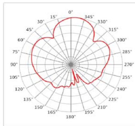
Azimuth @ 5.8GHz
