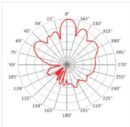
Elevation @ 5.8GHz
