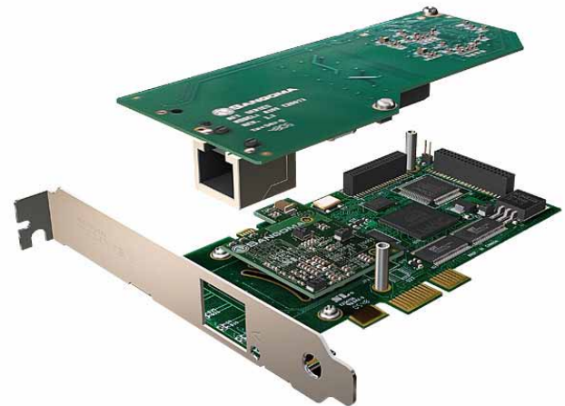
A101DE 1-port T1/E1/J1 shown with available echo canceller and PCI-Express interface
